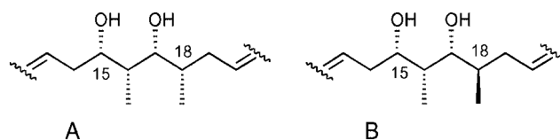
Figure 1. Relative configuration of C-15 to C-18 of cruentaren B predicted using Kishi's ^{13}\text{C} NMR chemical shift analysis. [11]
