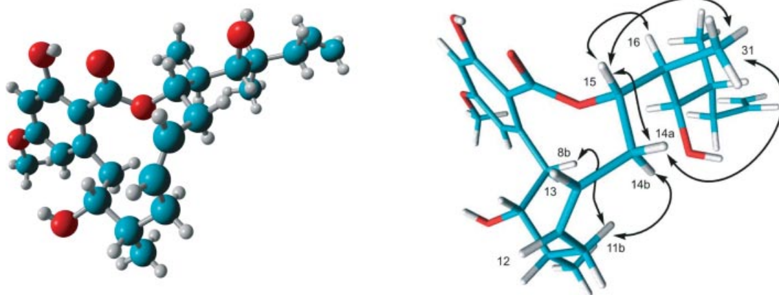
Figure 3. a) Crystal structure and b) proposed solution conformation with selected NOEs of 21,22- seco -cruentaren A ( 14 ).
