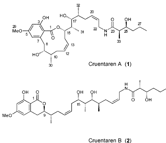
Figure 1. Relative configuration of C-15 to C-18 of cruentaren B predicted using Kishi's ^{13}\text{C} NMR chemical shift analysis. [11]
