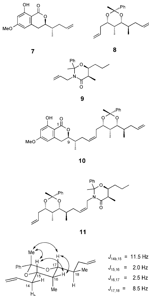
Figure 2. Relative configuration of 8 with selected NOEs and vicinal coupling constants.
